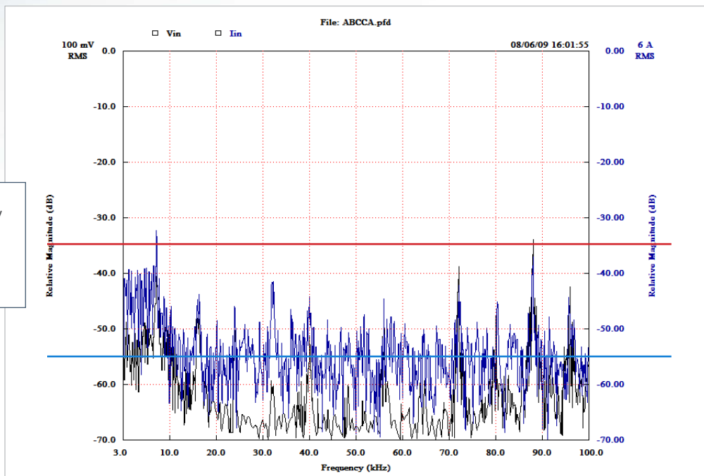
Figure 5: High frequency noise measured at VFD after EP installed
