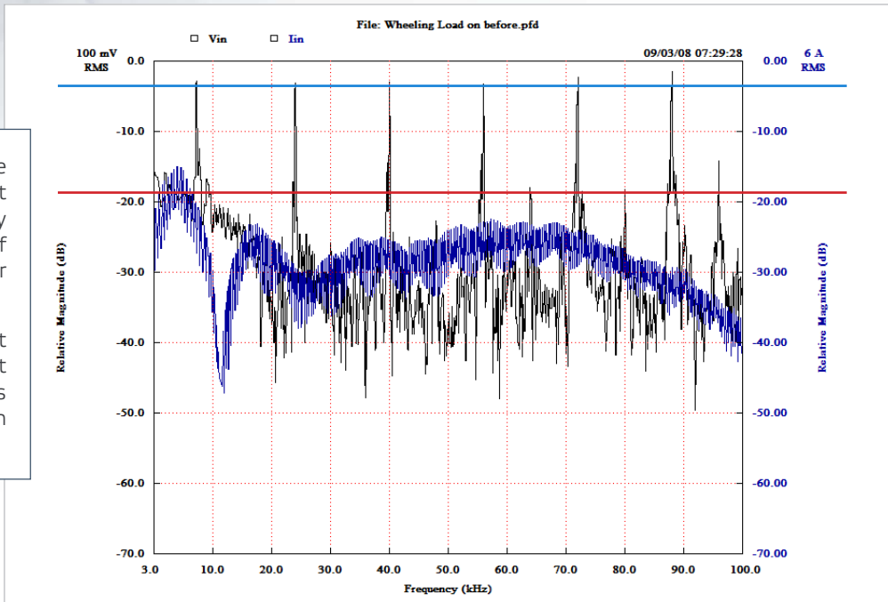
← Figure 4: Noise measured at VFD with the isolation transformer installed
